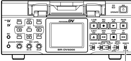
REMOTE/LOCAL switch
